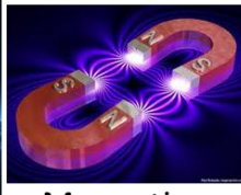
Magnetism
